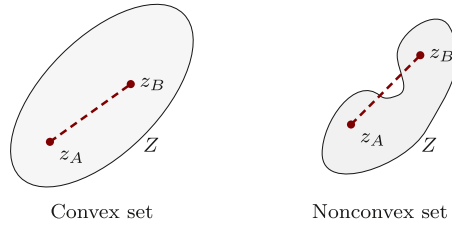
Convex set
