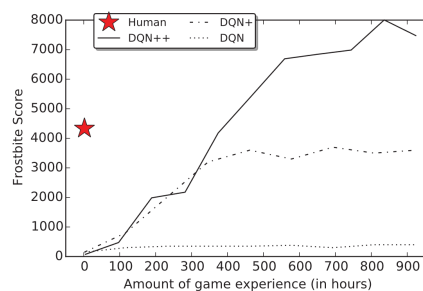
Figure 4.2: Comparison on the Frostbite game
