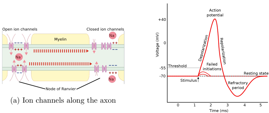
(b) Triggering of an action potential
