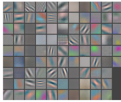
(a) AlexNet
