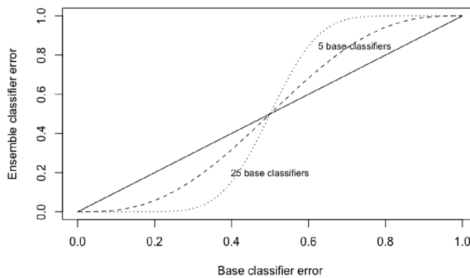
Figure 7.10: Relationship between the error of base classifiers and ensemble models
