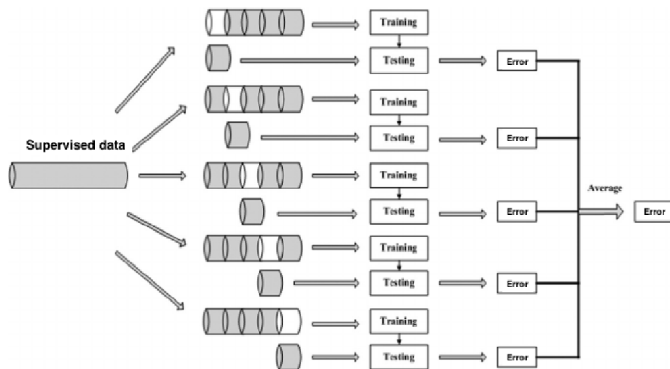
Figure 7.2: Cross-validation example
