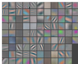
(a) AlexNet
