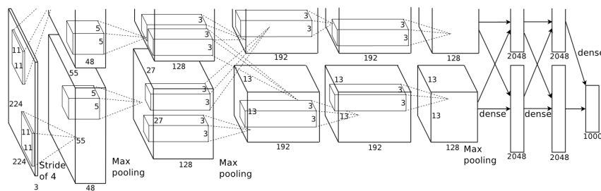
Figure 3.2: AlexNet architecture
