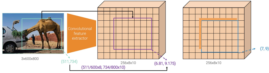
Figure 4.10: Project and snap operations
