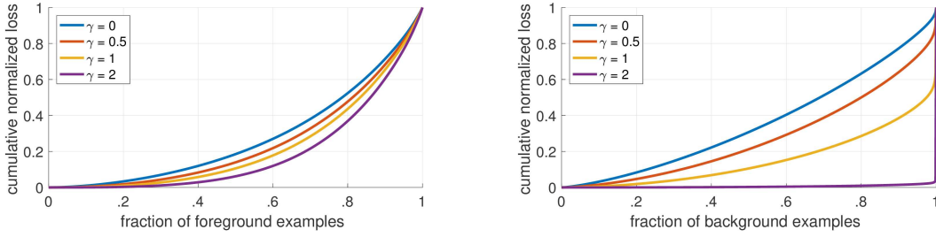
Figure 4.18: Cumulative loss contribution for varying \gamma of the focal loss.
