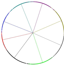
(a) Softmax
