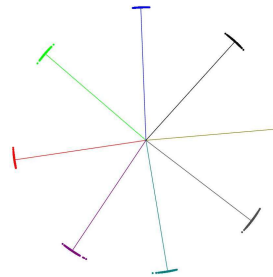
(b) ArcFace
