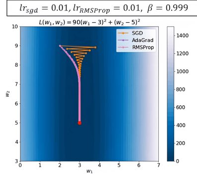
Figure 1.6: SGD vs AdaGrad vs RMSProp
