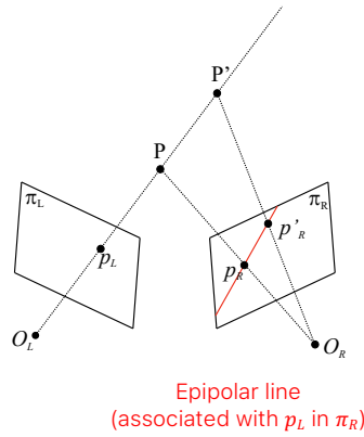
Figure 1.6: Example of epipolar geometry
