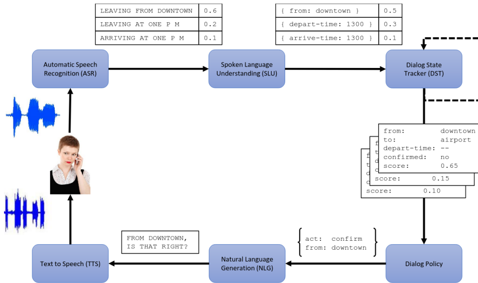
Figure A.2.: Example of components for a spoken dialog system
