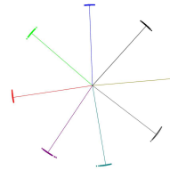
(b) ArcFace
