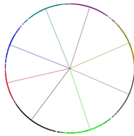
(a) Softmax
