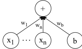
Figure 7.7: Example of perceptron
