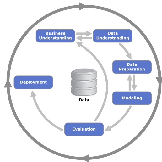
Figure 4.1: CRISP-DM workflow
