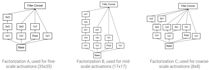
Figure 3.8: Inception-v3 modules
