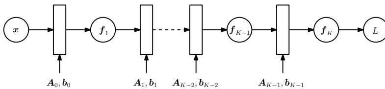
Figure 5.1: Forward pass
