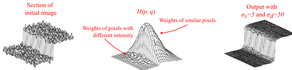
Figure 2.8: Example of bilateral filter application
