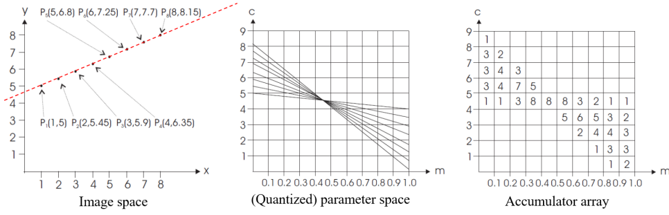
Figure 5.3: Example of line detection
