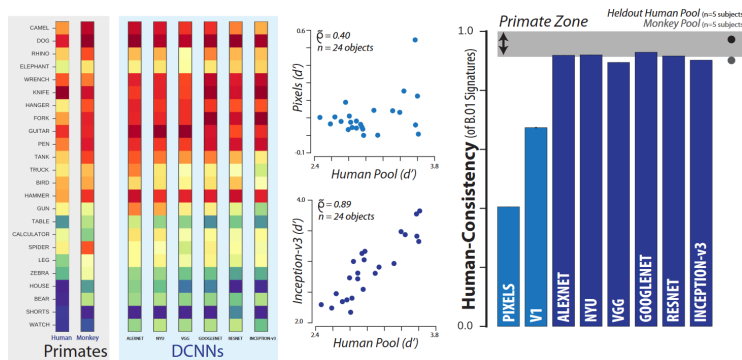
Figure 2.2: Object-level results. In the first part, warmer colors indicate a better classification.
