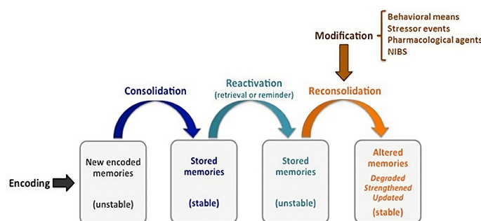
Figure 4.5: Memory flow
