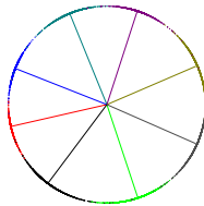
(a) Softmax
