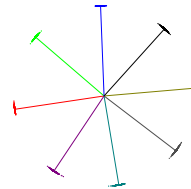
(b) ArcFace
