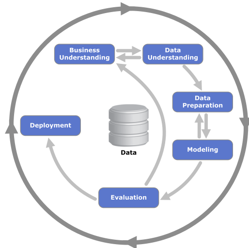
Figure 4.1: CRISP-DM workflow
