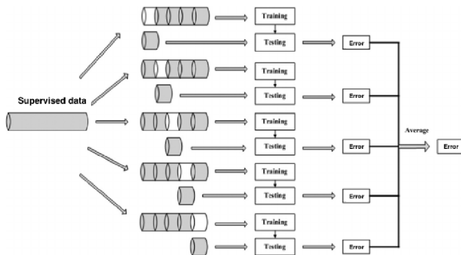
Figure 7.2: Cross-validation example
