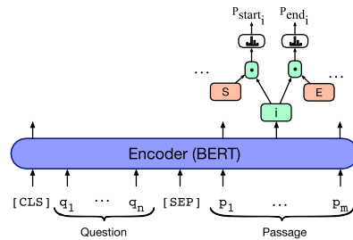
Figure 10.1.: Example of span labeling architecture
