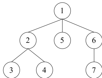
Figure 2.4: DFS visit order
