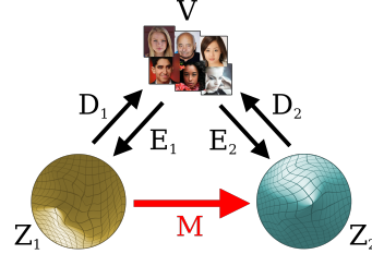
Figure 4.4: Example of mapping from a latent space Z_1 to a space Z_2 through M . The two spaces are evaluated on the visible space V .
