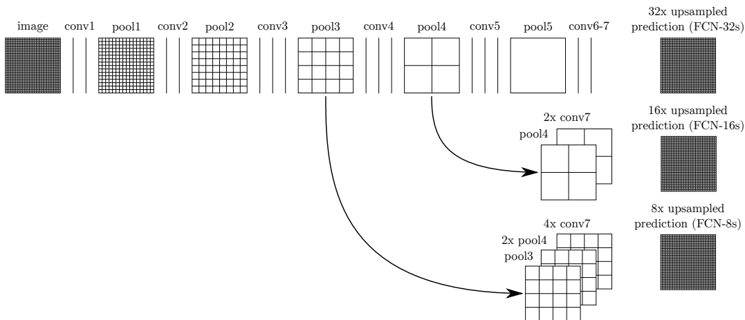
Figure 3.17: Examples of upsampling. The first row shows the upsampling process of the output (conv7) without skip connections. The second row shows the upsampling process with a skip connection from the second last pooling layer (pool4): the output (conv7) is partially upsampled to match the shape of the skip connection, then upsampling is done on their concatenation. The third row shows the upsampling process with skip connections up to the third last pooling layer (pool3).
