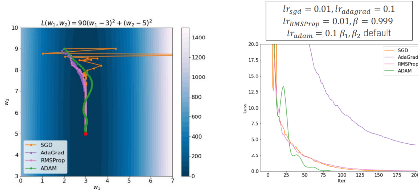
Figure 1.8: SGD vs AdaGrad vs RMSProp vs Adam with a smaller batch size
