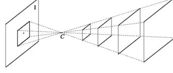
Figure 1.4: Projection from scene and image points
