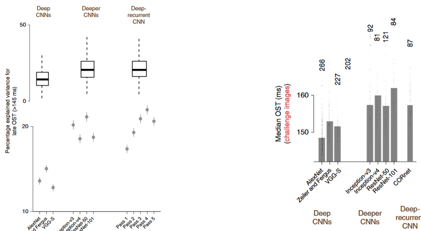
(b) Number (on top) and median OST (bars) of the unsolved images for each model
