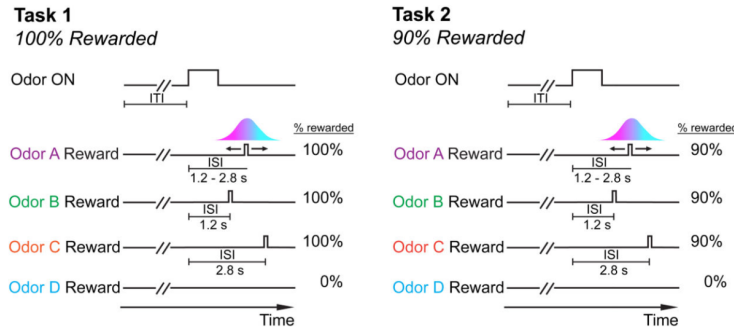
Figure 3.9: Tasks representation
