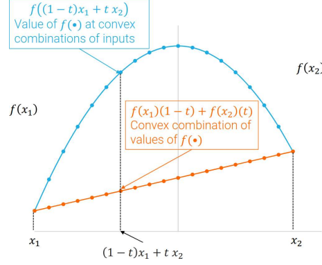
Figure 8.4: Visualization of the Jensen's inequality
