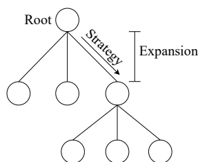
Figure 2.1: Search tree
