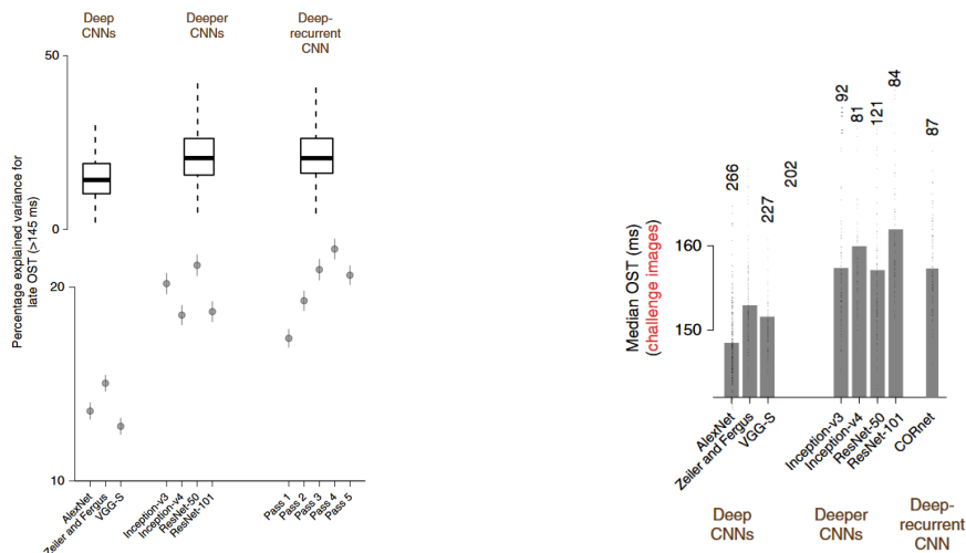
(a) Predictivity for deep, deeper and recurrent CNNs (b) Number (on top) and median OST (bars) of the unsolved images for each model
