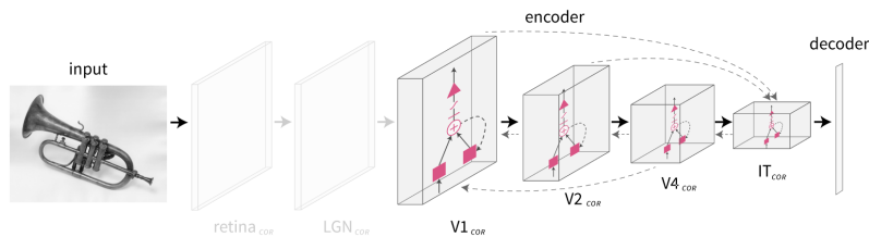
Figure 2.4: Architecture of CORnet
