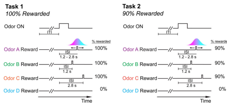
Figure 3.9: Tasks representation
