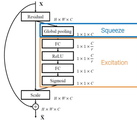
Figure 2.5: SE-ResNet module
